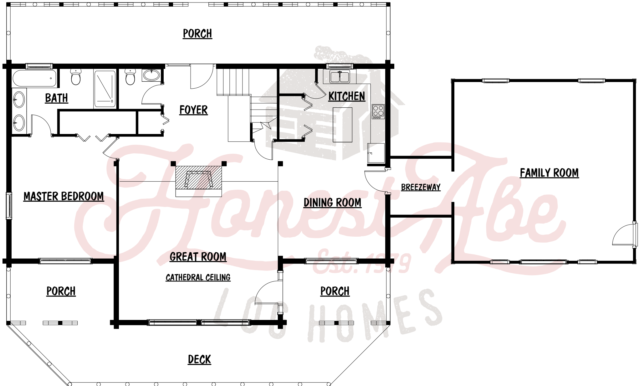
Bellewood - First Floor
